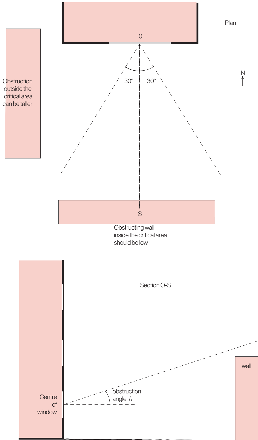
Figure 35: For passive solar gains in winter the sector AOB 30° either side of due south is important. To guarantee winter sun from this sector, obstructions within it should not subtend more than the critical angle h when measured in section. Table 1 gives values for h .
